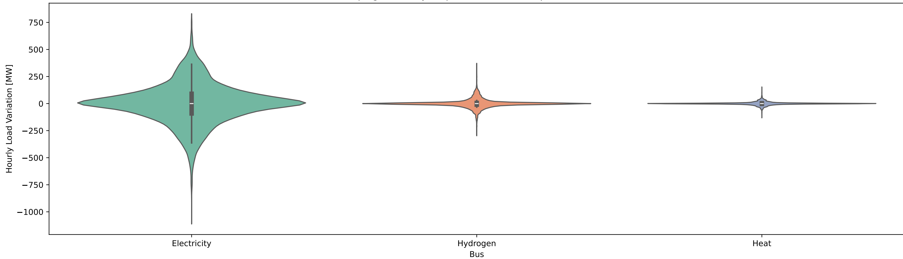
Ramping Flexibility Requirements (1h Ramps for All Buses)
